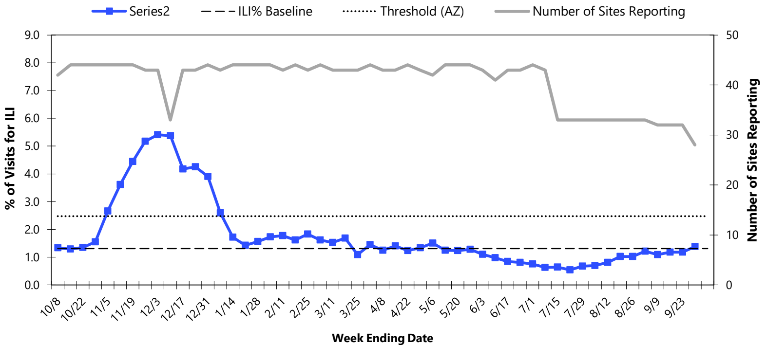
Percentage of Visits for ILI at Sentinel Providers, 2022-2023, Arizona
